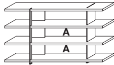
LB1972 width 2000 depth 416 height 1120
