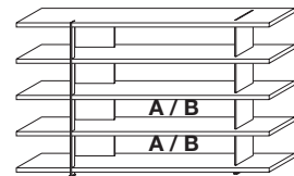
LB2403 width 2400 depth 416 height 1465
