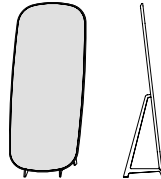
SP075C width 750 depth 420 height1800
