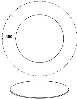
LSVL160 LSVM160 Ø 1600 height 20
