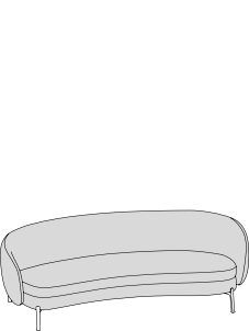
OBDI222 width 2220 depth 1025 height 690/835 seat height 400 seat depth 635/550
